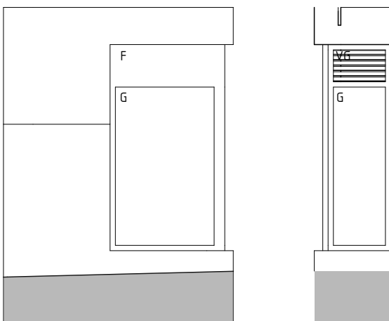
FASAD MOT ANNA WITHLOCKS GATA
